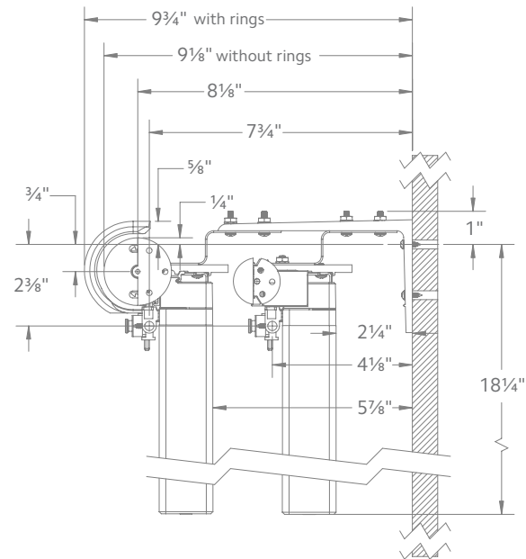
2" & 1 3/8" DOUBLE MOUNT
